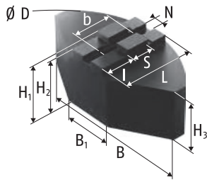
Weiche Segmentbacken SFA-SM Stahl 16MnCr5 einsatzhärtnbar Soft Full Grip Jaws SFA-SM Steel 16MnCr5 suitable for case hardening
