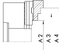
Grundbackenstellung I Position of base jaws I
