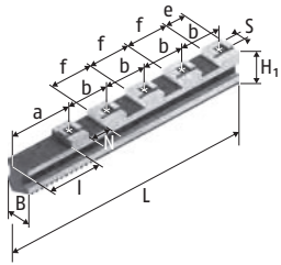
Grundbacken SFGF-L Base Jaws SFGF-L
