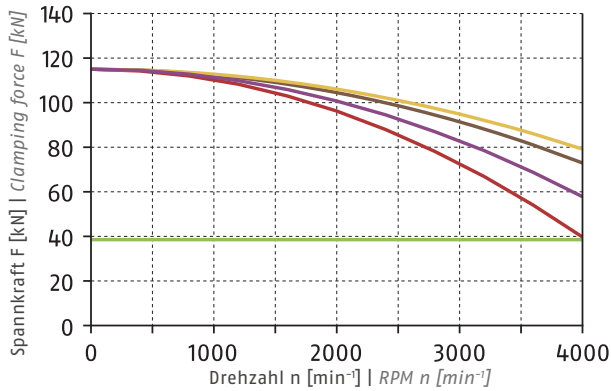
Clamping force-RPM-diagram
