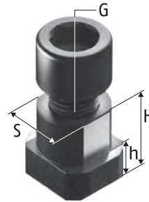
Nutensteine NS T-Nuts NS
